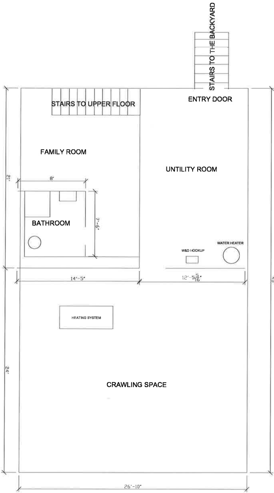
Floor Plan drafted by Youssef Kubis, Owner LOWER FLOOR (WITHOUT THE CRAWLING SPACE): 567 SF
